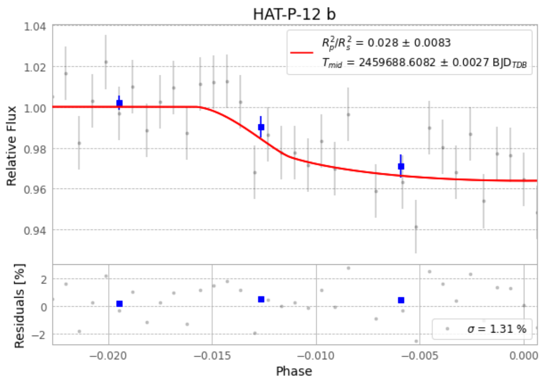
Figure 1 — FinalLightCurve_HAT-P-12 b_2022-04-21.png (SHA-256 652bfc2b559ba447...)
