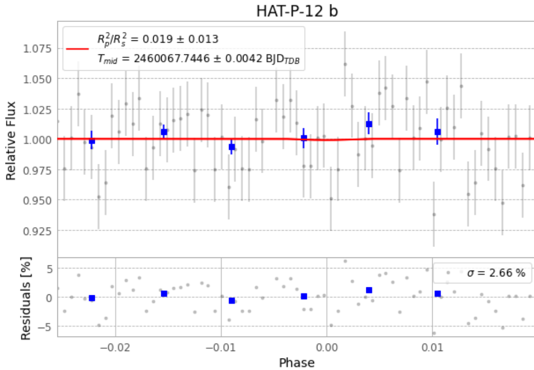
Figure 1 — FinalLightCurve_HAT-P-12 b_2023-05-02.png (SHA-256 673f224bf77f1d6b...)
