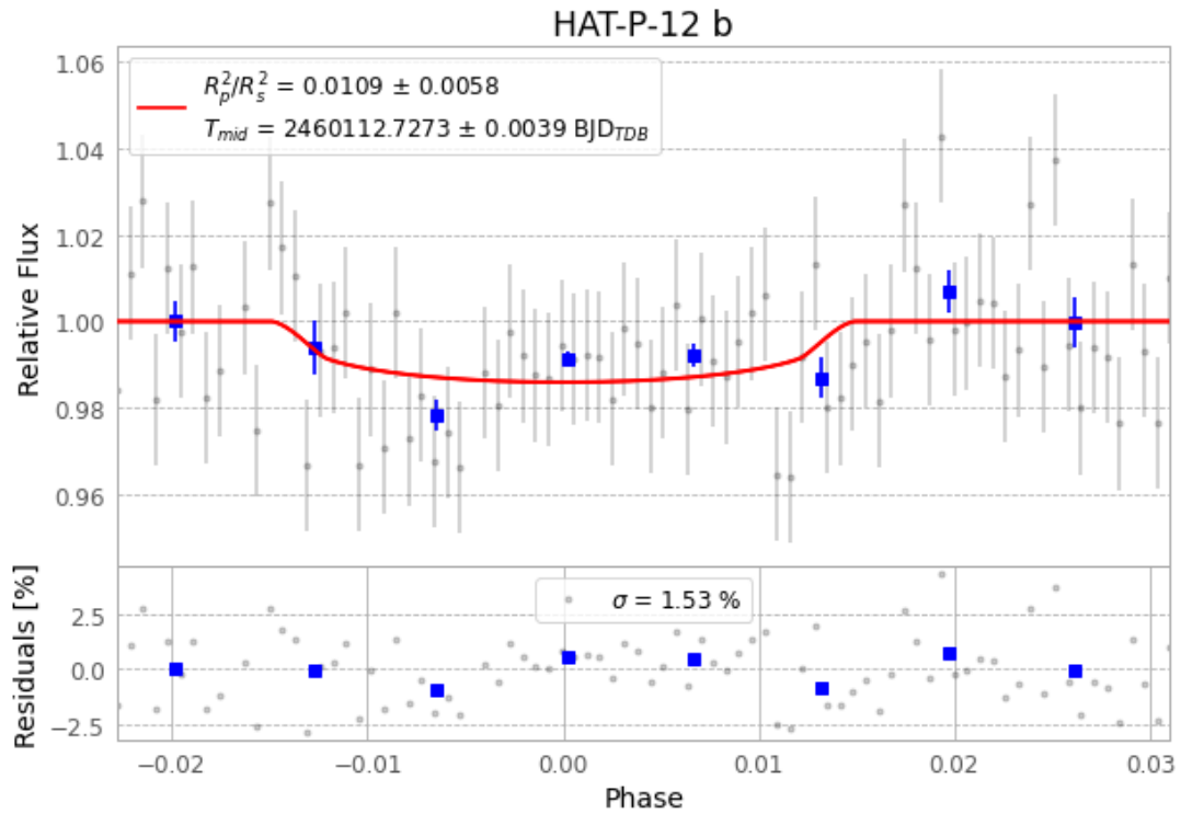
Figure 1 — FinalLightCurve_HAT-P-12 b_2023-06-16.png (SHA-256 cb3d90492c247f46...)
