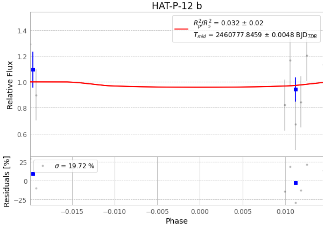
Figure 1 — FinalLightCurve_HAT-P-12 b_2025-04-11.png (SHA-256 68c18edd88313766...)
