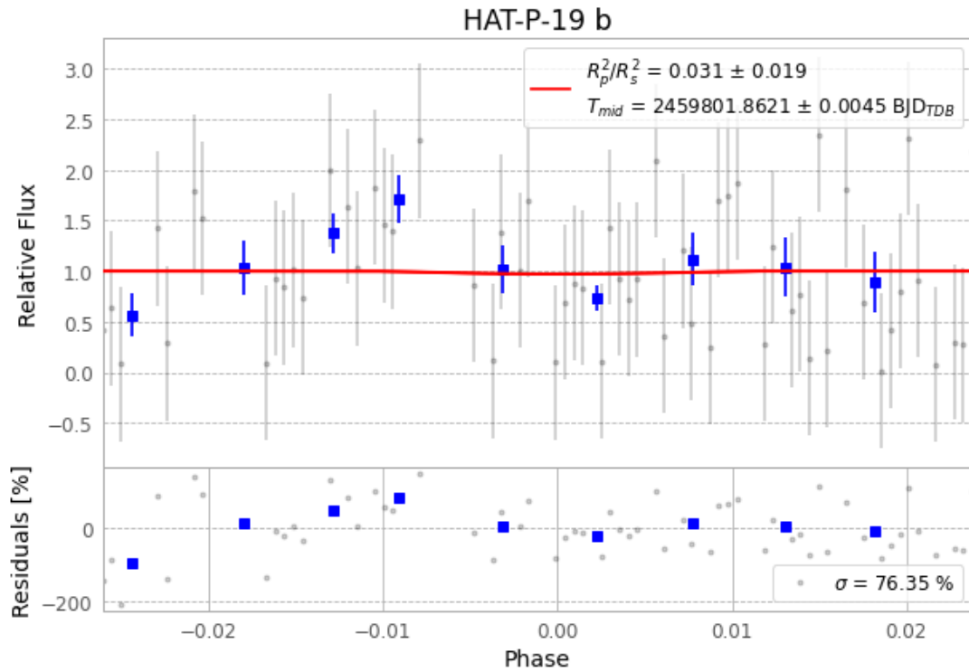
Figure 1 — FinalLightCurve_HAT-P-19 b_2022-08-09.png (SHA-256 b76e7d0e3ecb8be5...)
