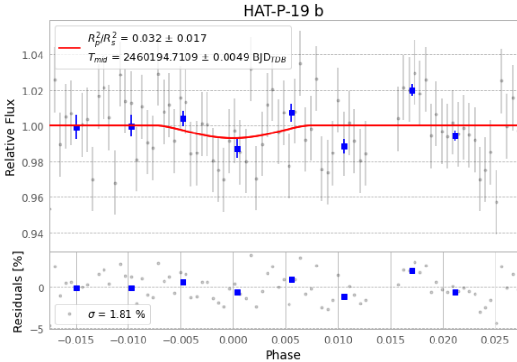
Figure 1 — FinalLightCurve_HAT-P-19 b_2023-09-06.png (SHA-256 ebcd4c8083ecf7b3...)
