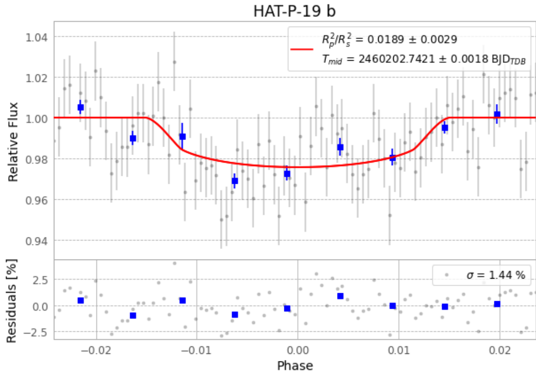
Figure 1 — FinalLightCurve_HAT-P-19 b_2023-09-14.png (SHA-256 f675616ea08ae4f2...)
