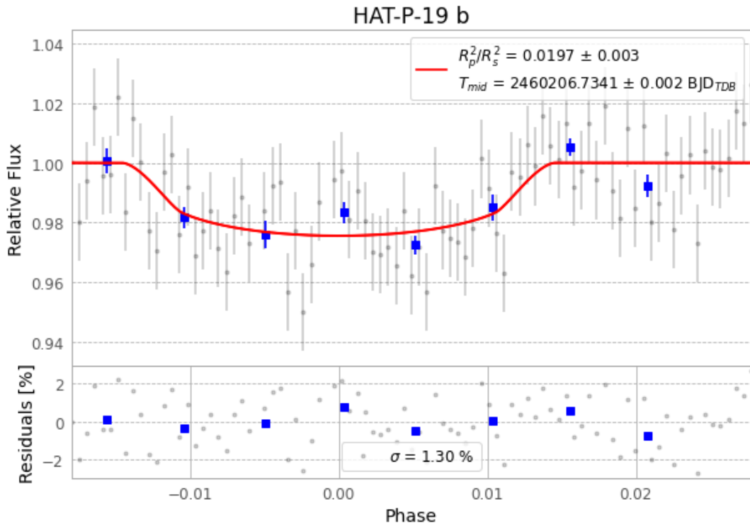
Figure 1 — FinalLightCurve_HAT-P-19 b_2023-09-18.png (SHA-256 fe9af909823a76e0...)
