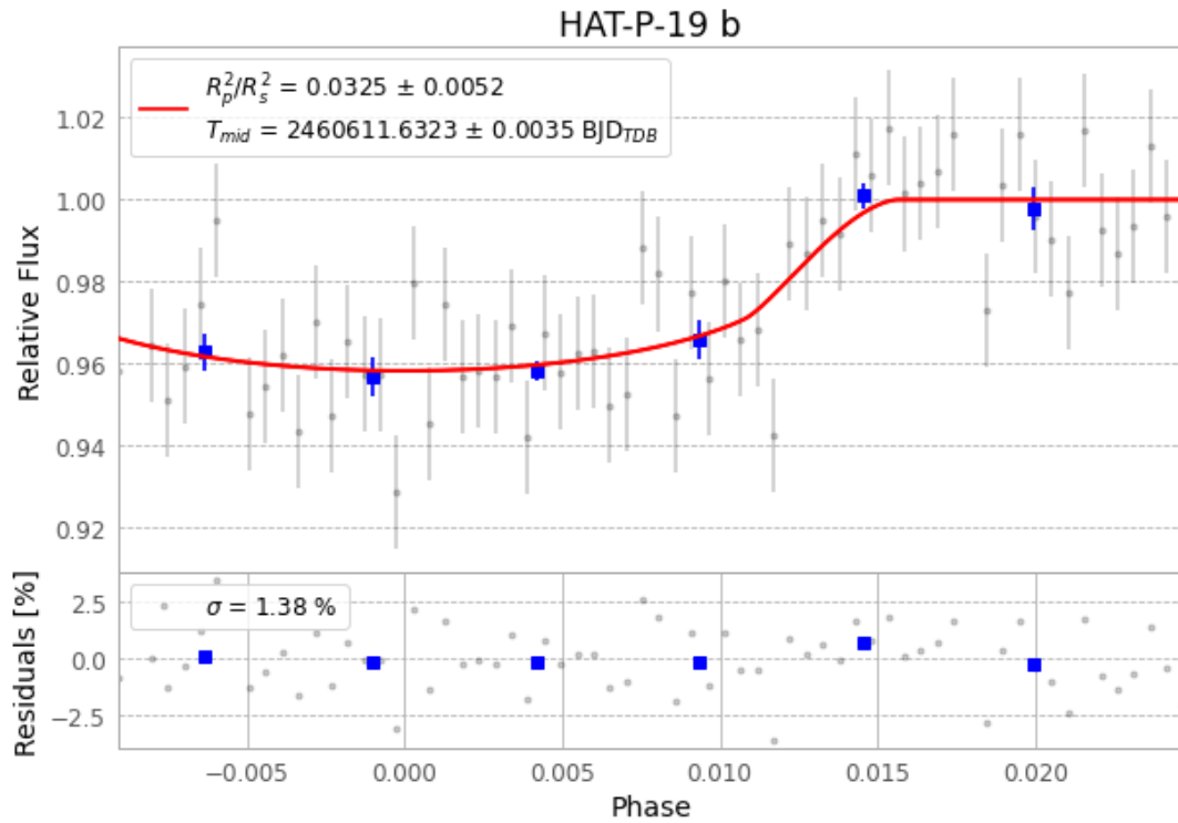
Figure 1 — FinalLightCurve_HAT-P-19 b_2024-10-27.png (SHA-256 878117a604c65e7c...)
