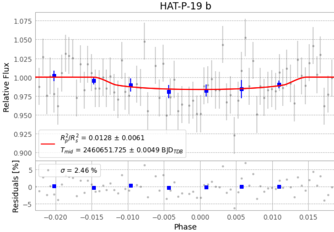
Figure 1 — FinalLightCurve_HAT-P-19 b_2024-12-06.png (SHA-256 65f729c19993c3e5...)
