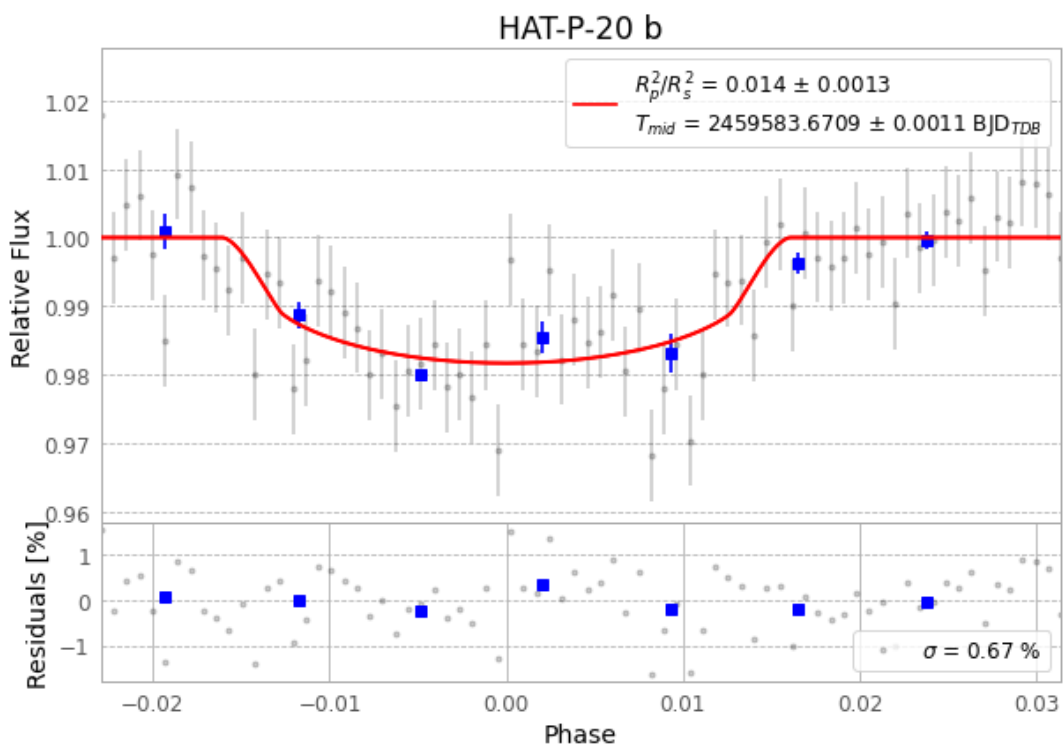
Figure 1 — FinalLightCurve_HAT-P-20 b_2022-01-03.png (SHA-256 691e683e10508b6d...)
