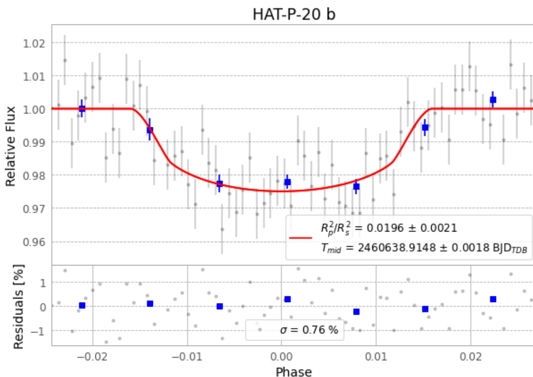
Figure 1 — FinalLightCurve_HAT-P-20 b_2024-11-24.png (SHA-256 788747d95d8191d5...)
