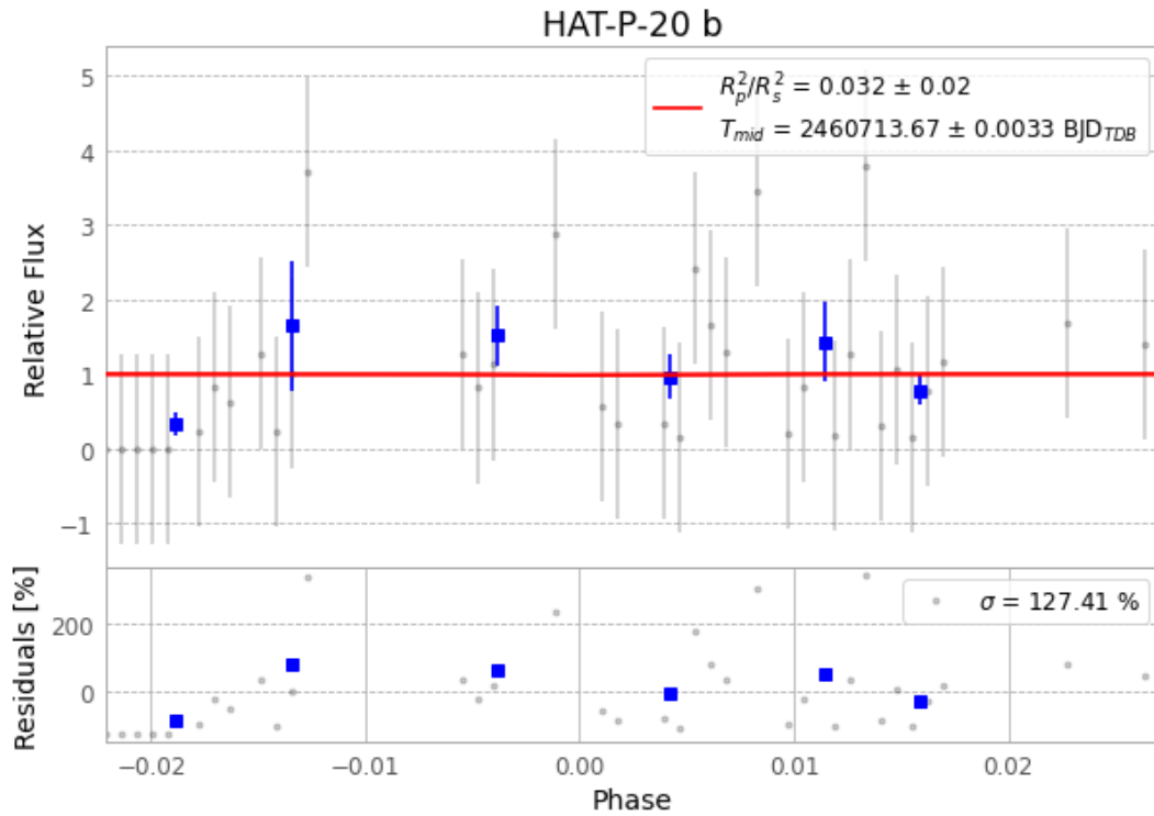
Figure 1 — FinalLightCurve_HAT-P-20 b_2025-02-06.png (SHA-256 463e2032cf98eb1c...)
