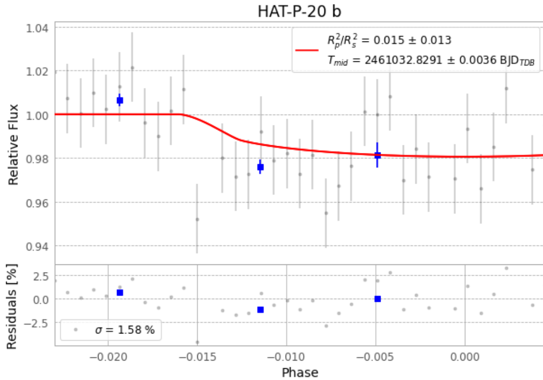
Figure 1 — FinalLightCurve_HAT-P-20 b_2025-12-22.png (SHA-256 49312aa8e326ed0c...)
