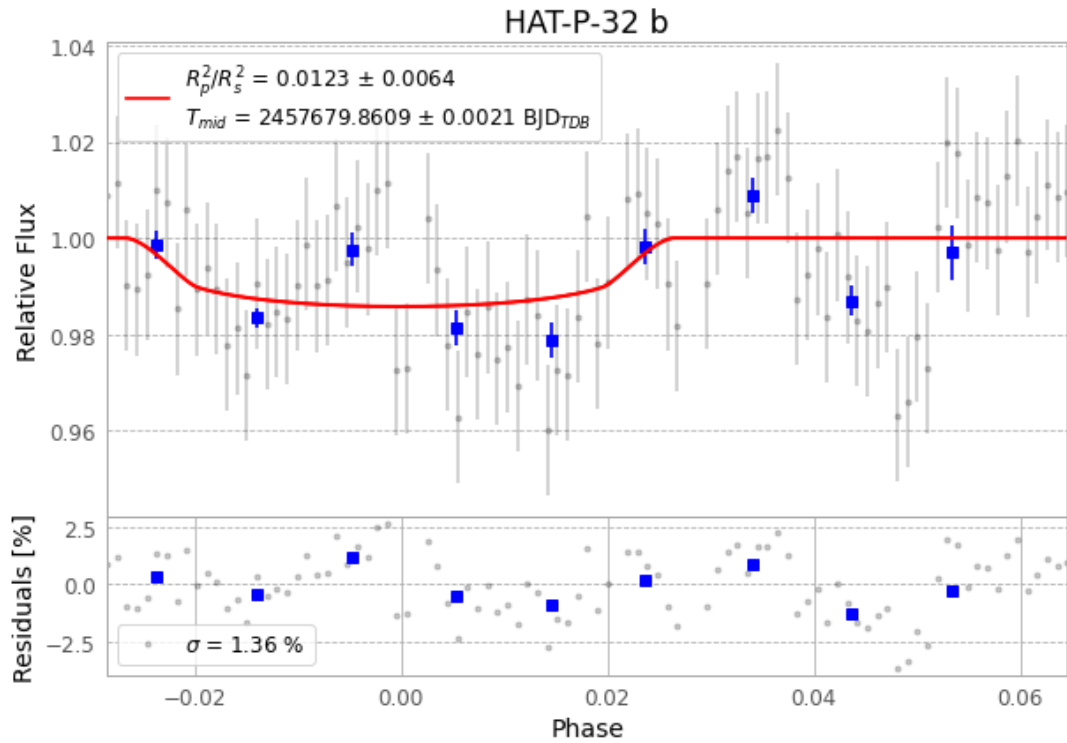
Figure 1 — FinalLightCurve_HAT-P-32 b_2016-10-18.png (SHA-256 c54b47b1c853173f...)
