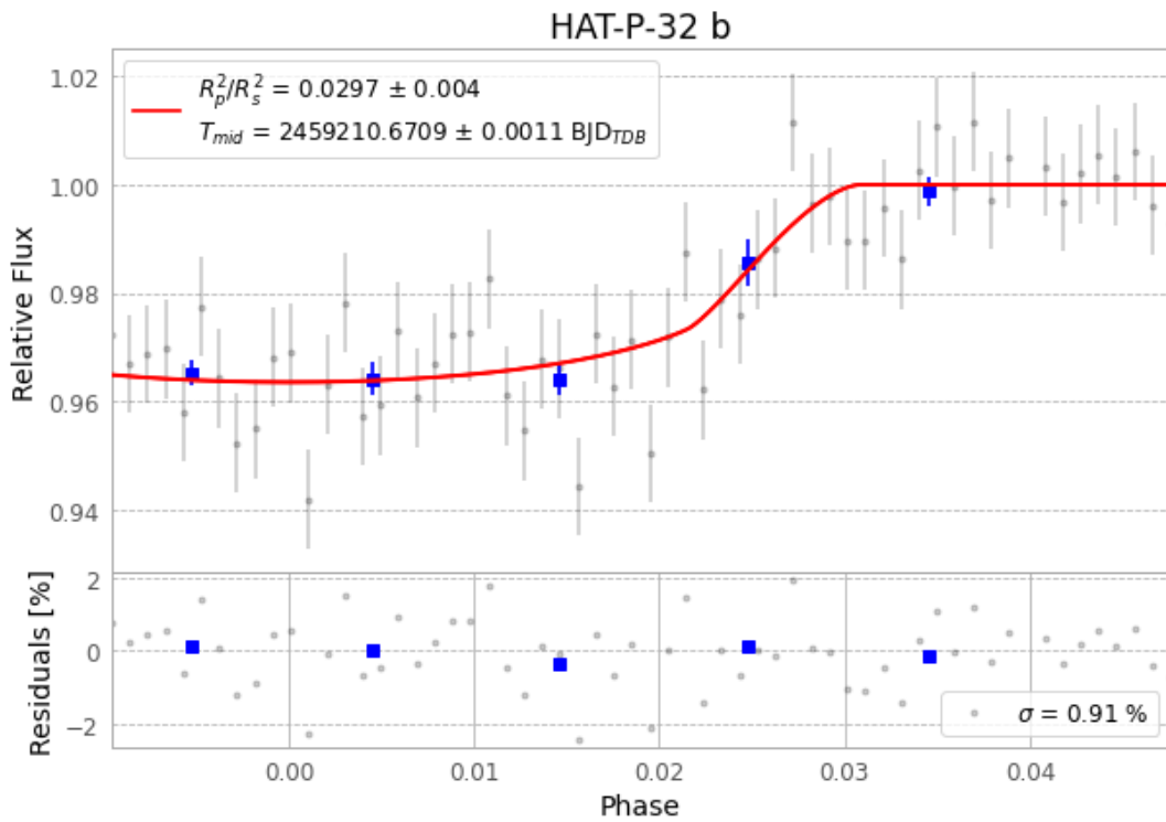
Figure 1 — FinalLightCurve_HAT-P-32 b_2020-12-26.png (SHA-256 a73a86954291348e...)
