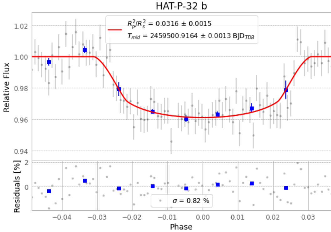
Figure 1 — FinalLightCurve_HAT-P-32 b_2021-10-13.png (SHA-256 803b4fd926192550...)
