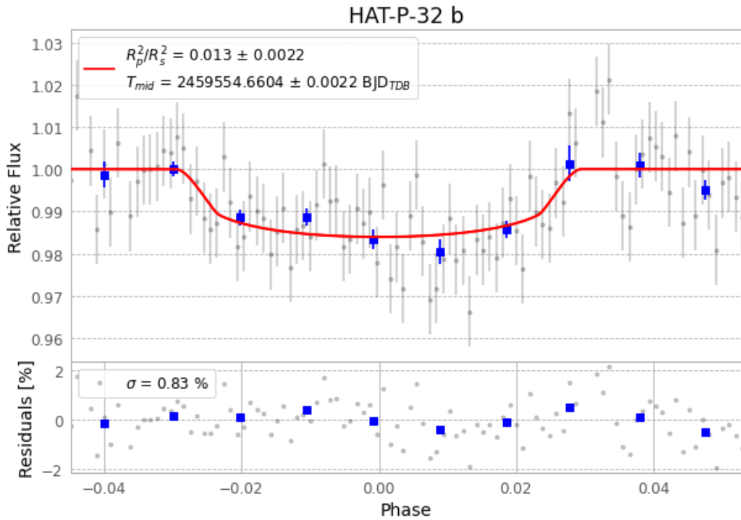
Figure 1 — FinalLightCurve_HAT-P-32 b_2021-12-05.png (SHA-256 a1c7768f80b2d001...)
