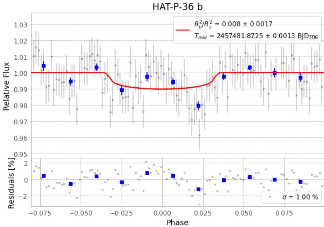
Figure 1 — FinalLightCurve_HAT-P-36 b_2016-04-02.png (SHA-256 9c85eec1b02e9ae3...)
