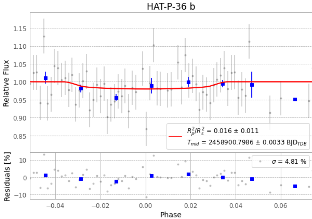
Figure 1 — FinalLightCurve_HAT-P-36 b_2020-02-20.png (SHA-256 1c28453791bbfa47...)
