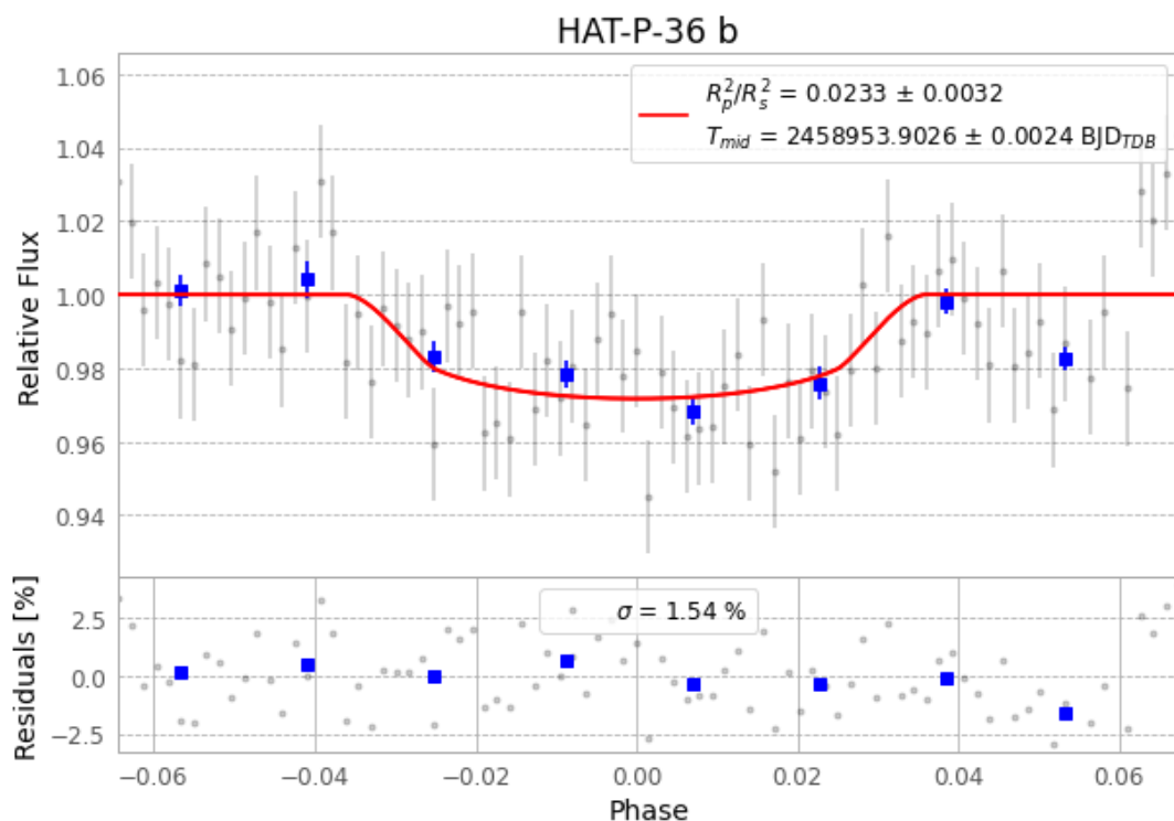
Figure 1 — FinalLightCurve_HAT-P-36 b_2020-04-14.png (SHA-256 e3d3691c34c9bfa1...)
