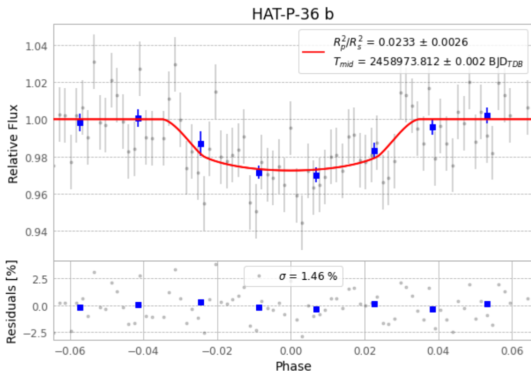
Figure 1 — FinalLightCurve_HAT-P-36 b_2020-05-03.png (SHA-256 aac12195fd3f67ba...)
