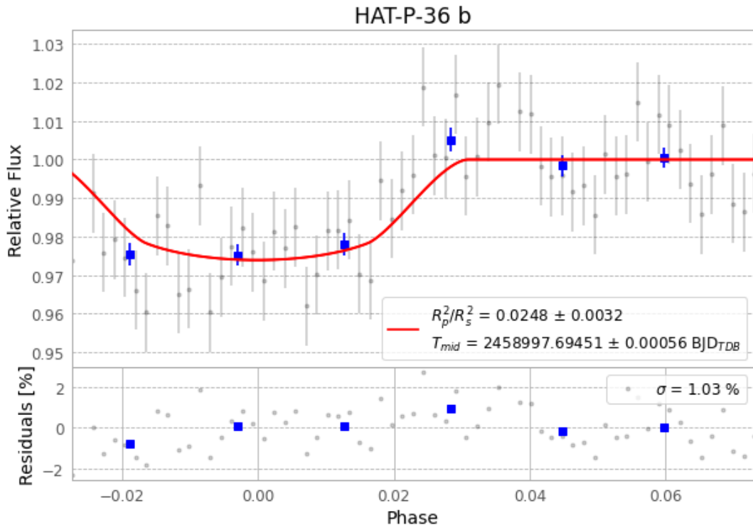
Figure 1 — FinalLightCurve_HAT-P-36 b_2020-05-27.png (SHA-256 f56566a4e1198ac2...)
