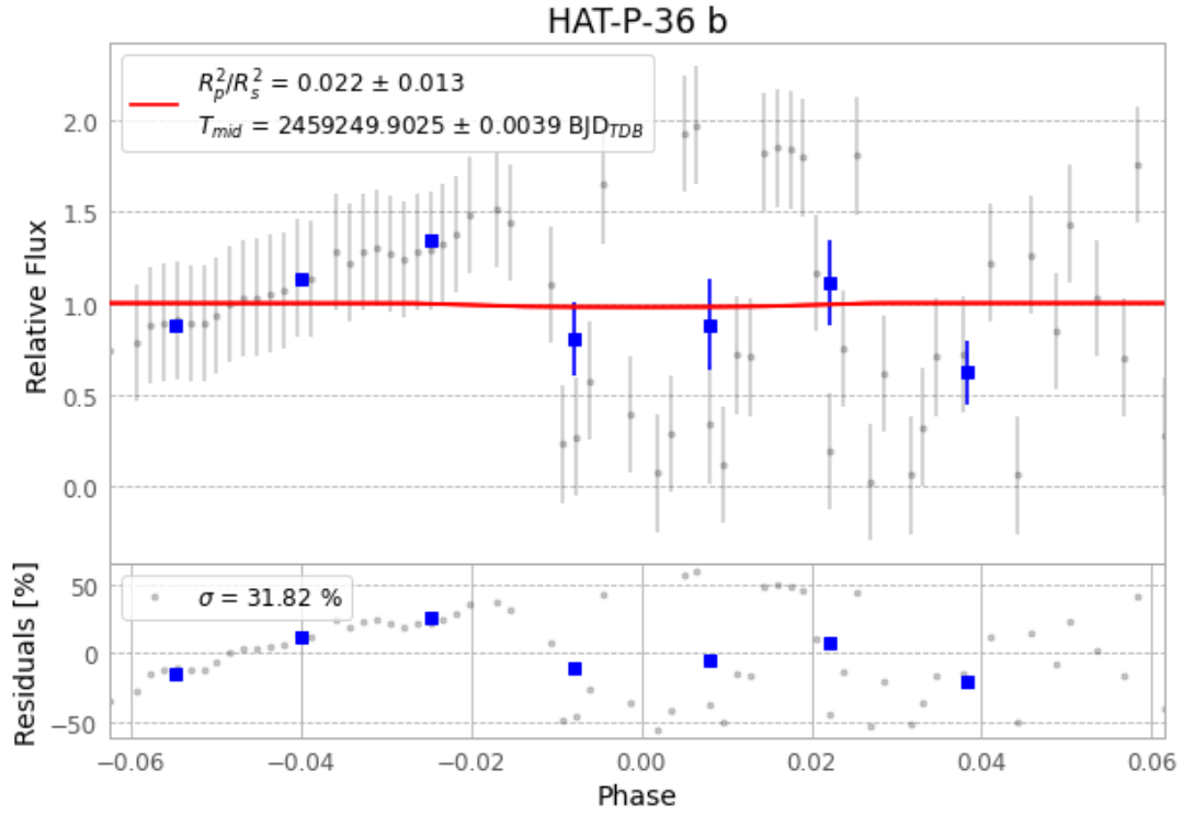
Figure 1 — FinalLightCurve_HAT-P-36 b_2021-02-04.png (SHA-256 44997a537e0d5056...)
