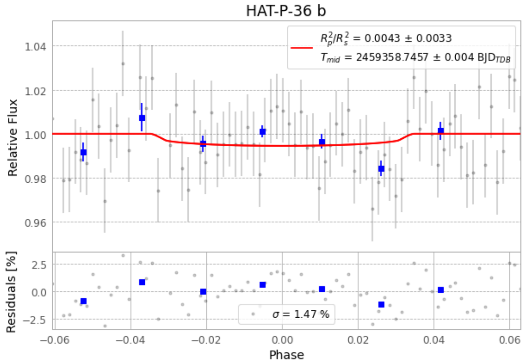
Figure 1 — FinalLightCurve_HAT-P-36 b_2021-05-23.png (SHA-256 fea044bd90f3b4f2...)
