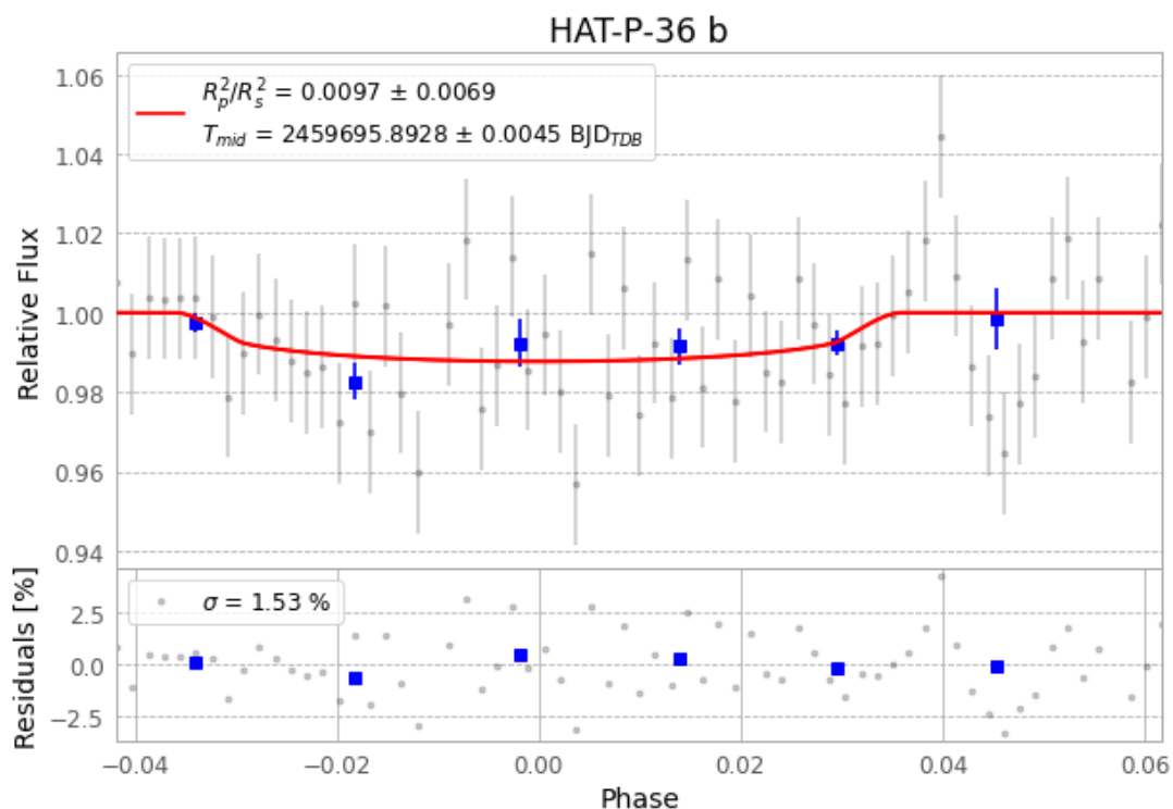
Figure 1 — FinalLightCurve_HAT-P-36 b_2022-04-26.png (SHA-256 97e5b8bf7f6df7d7...)
