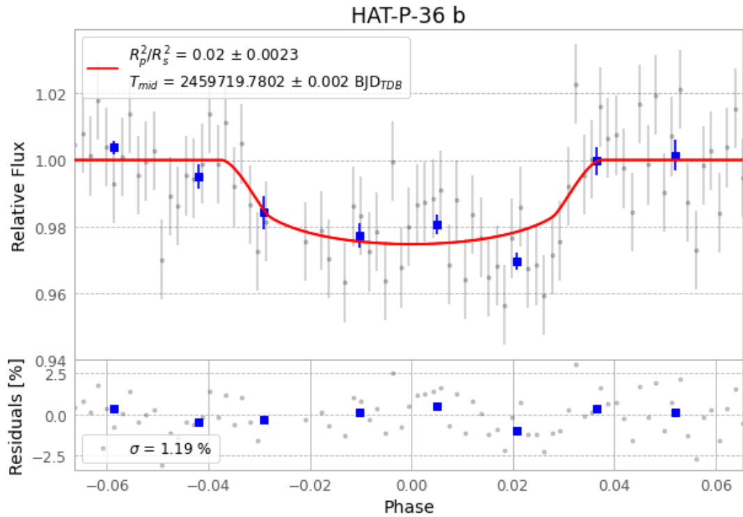
Figure 1 — FinalLightCurve_HAT-P-36 b_2022-05-19.png (SHA-256 257a36c2270a3889...)
