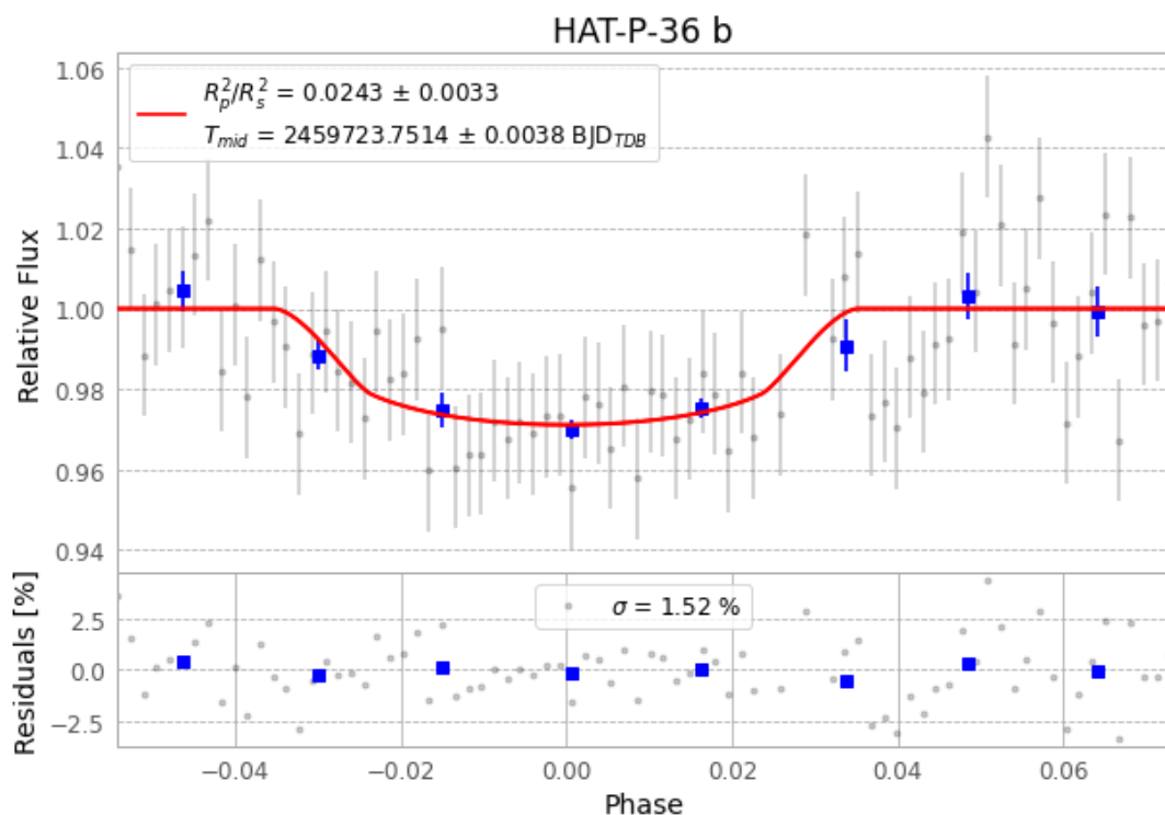
Figure 1 — FinalLightCurve_HAT-P-36 b_2022-05-23.png (SHA-256 e2a3a108a31cec08...)
