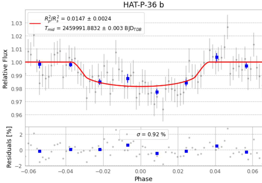
Figure 1 — FinalLightCurve_HAT-P-36 b_2023-02-16.png (SHA-256 e17d1ae3776f0c3a...)
