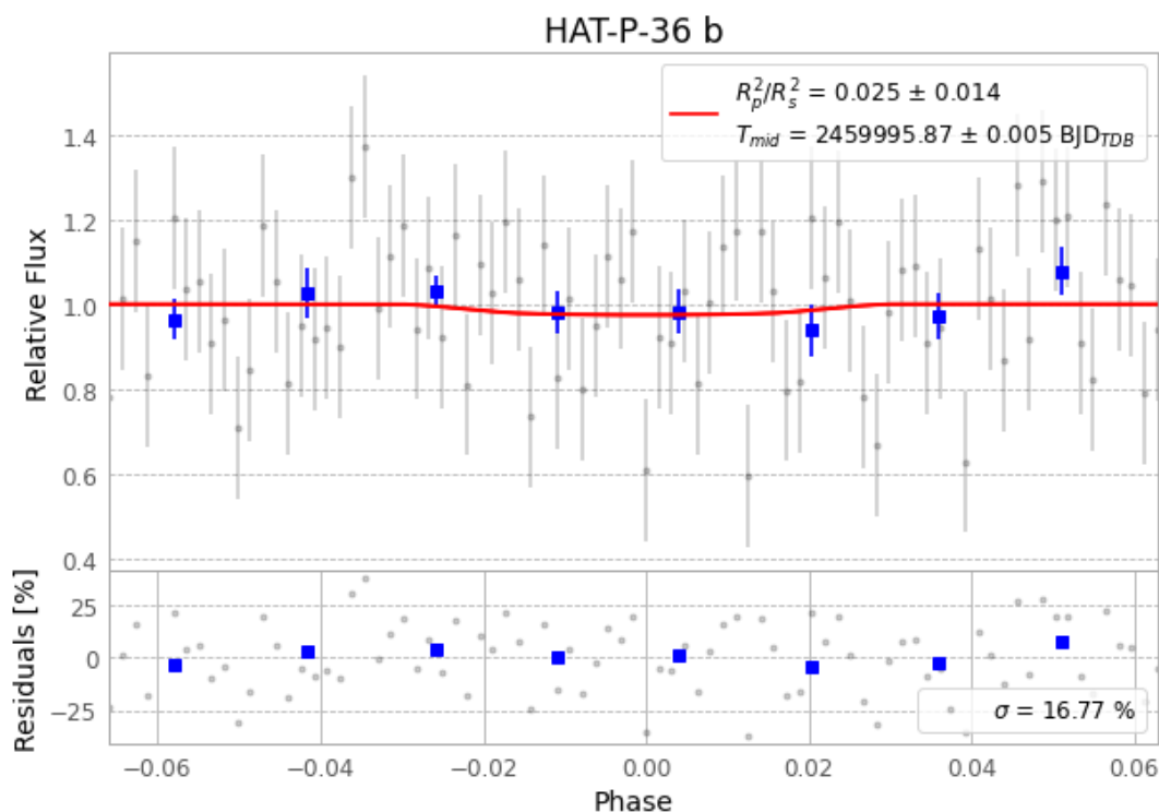
Figure 1 — FinalLightCurve_HAT-P-36 b_2023-02-19.png (SHA-256 cf7e57d66abe8cfd...)
