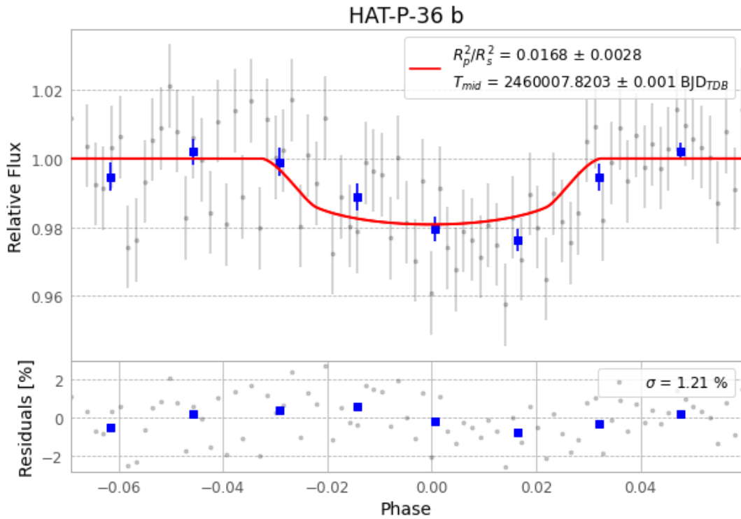
Figure 1 — FinalLightCurve_HAT-P-36 b_2023-03-03.png (SHA-256 7947531fffd6159e...)
