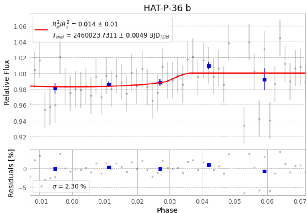
Figure 1 — FinalLightCurve_HAT-P-36 b_2023-03-19.png (SHA-256 34d41e1b8eb250cb...)
