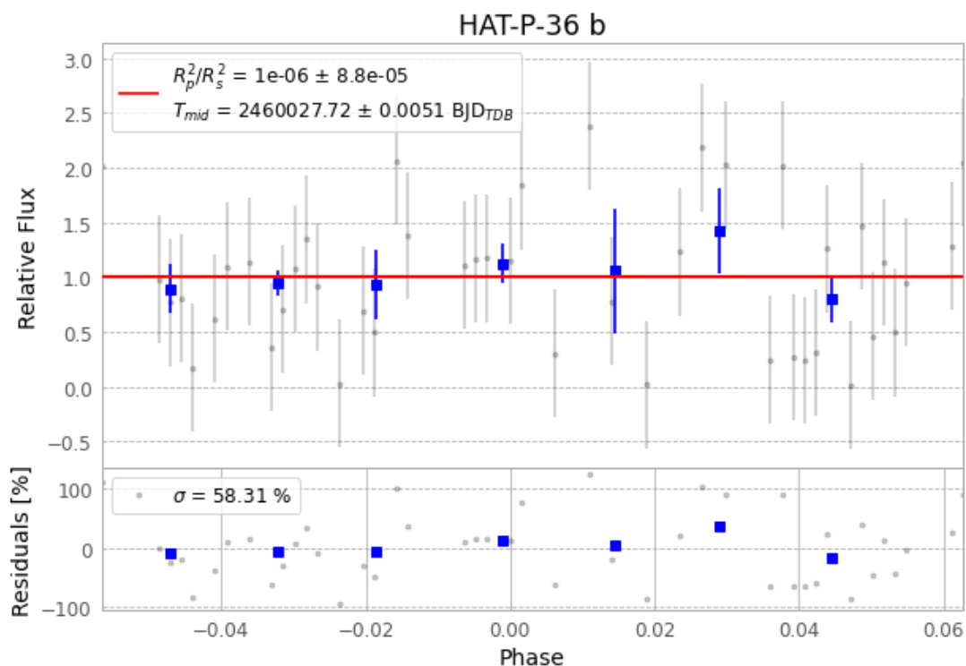
Figure 1 — FinalLightCurve_HAT-P-36 b_2023-03-23.png (SHA-256 1349b50ff8db8551...)
