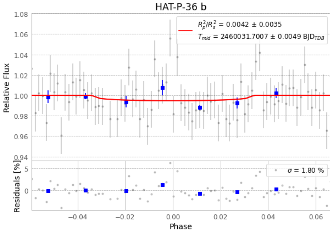
Figure 1 — FinalLightCurve_HAT-P-36 b_2023-03-27.png (SHA-256 eeb98718e74a3755...)
