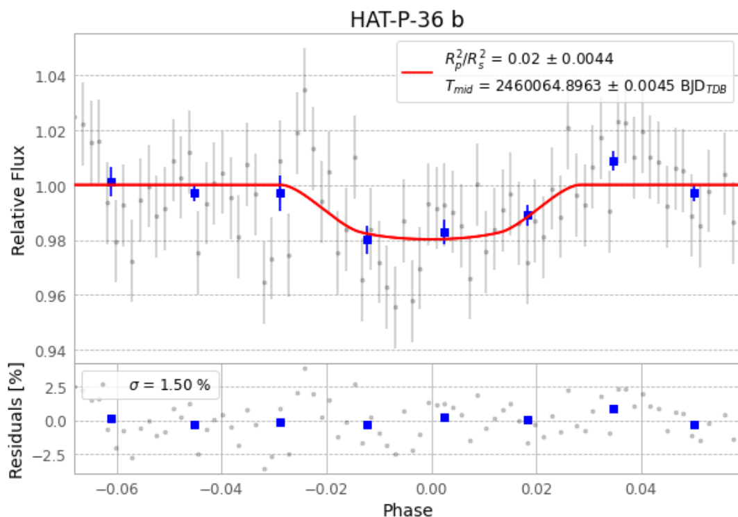
Figure 1 — FinalLightCurve_HAT-P-36 b_2023-04-30.png (SHA-256 093c849bf27b6fd5...)
