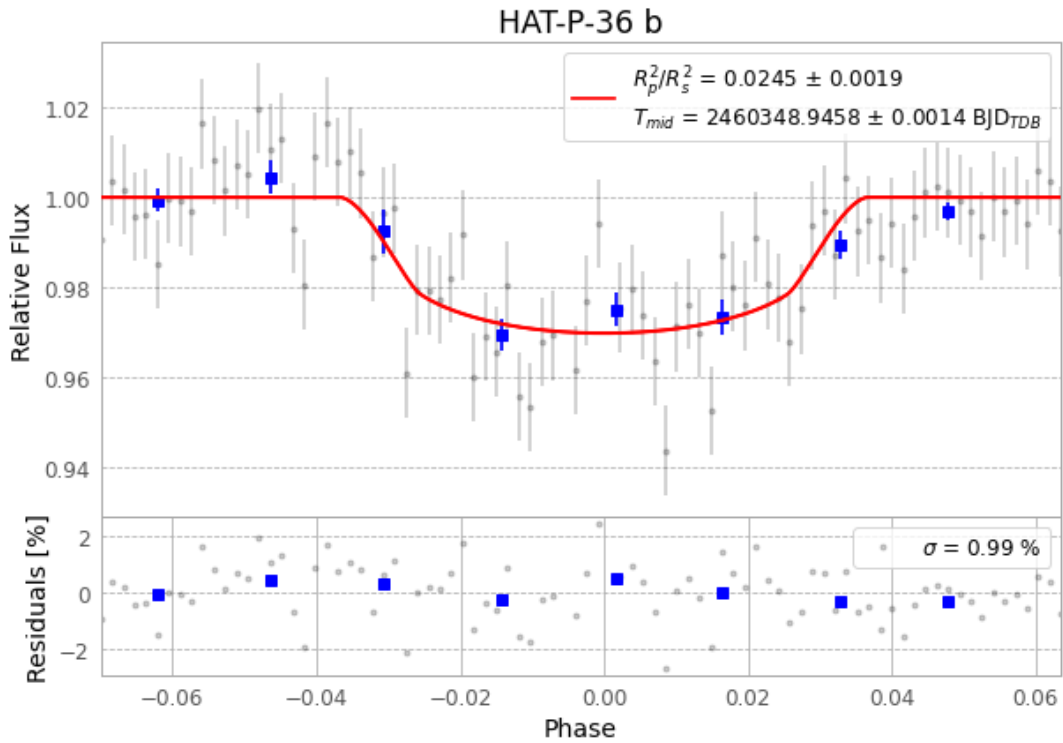
Figure 1 — FinalLightCurve_HAT-P-36 b_2024-02-08.png (SHA-256 f1c703021963f373...)
