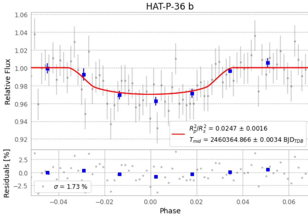
Figure 1 — FinalLightCurve_HAT-P-36 b_2024-02-24.png (SHA-256 623dc10141f9671b...)
