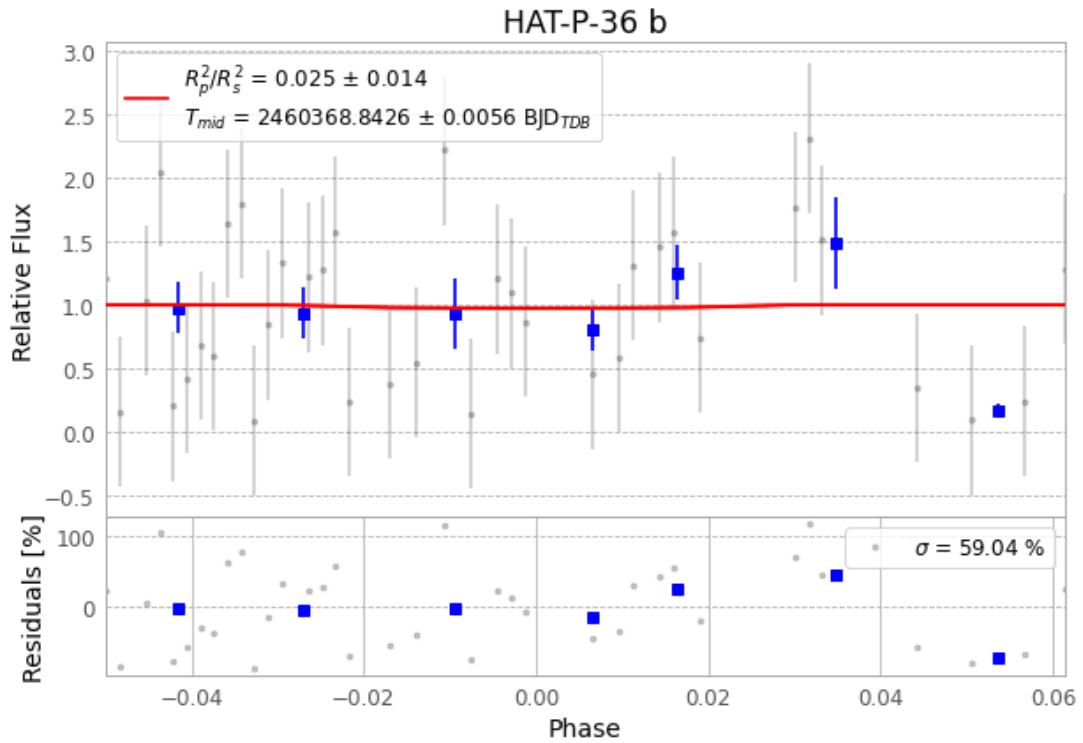
Figure 1 — FinalLightCurve_HAT-P-36 b_2024-02-27.png (SHA-256 1aba4cae24fb42c0...)
