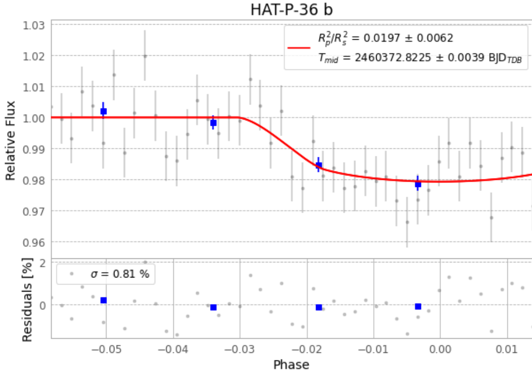
Figure 1 — FinalLightCurve_HAT-P-36 b_2024-03-02.png (SHA-256 438d3c3b80ecbef1...)
