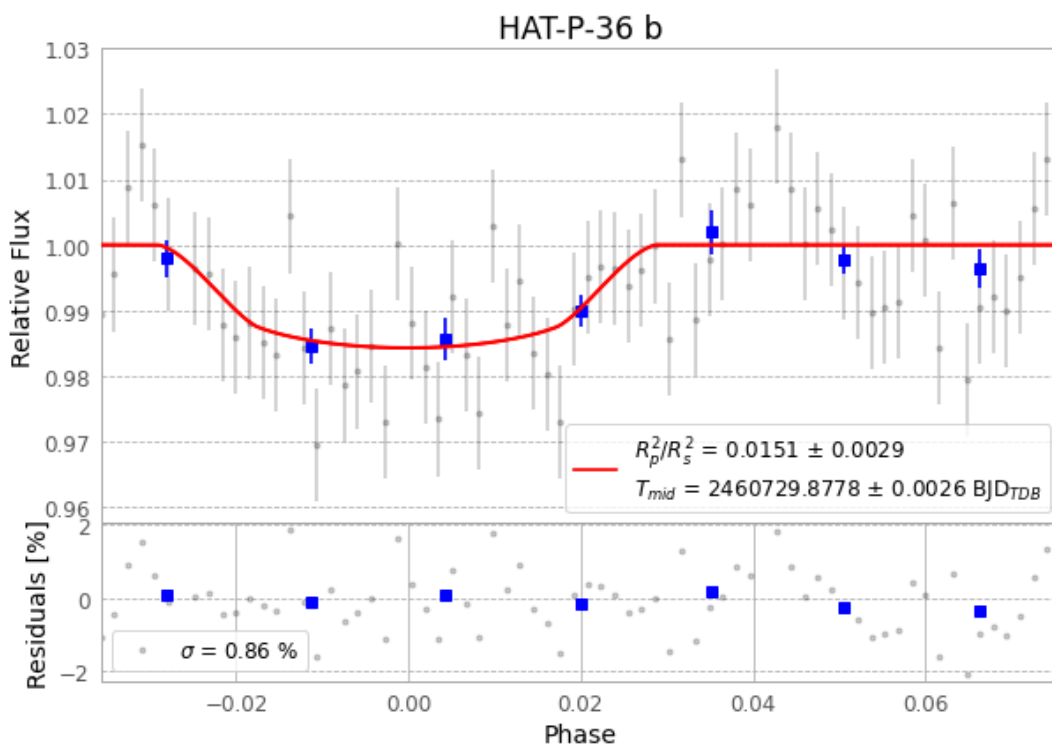
Figure 1 — FinalLightCurve_HAT-P-36 b_2025-02-23.png (SHA-256 2433a498edaabb4b...)
