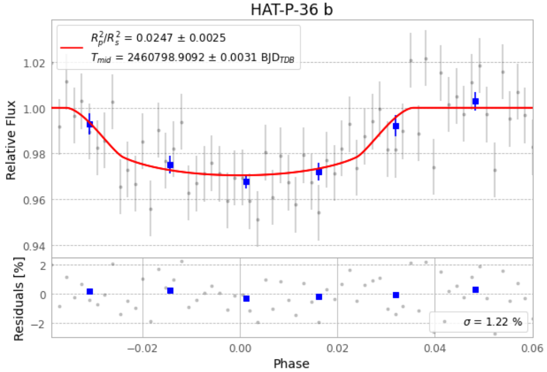
Figure 1 — FinalLightCurve_HAT-P-36 b_2025-05-03.png (SHA-256 4bc1abdacf4b9baa...)
