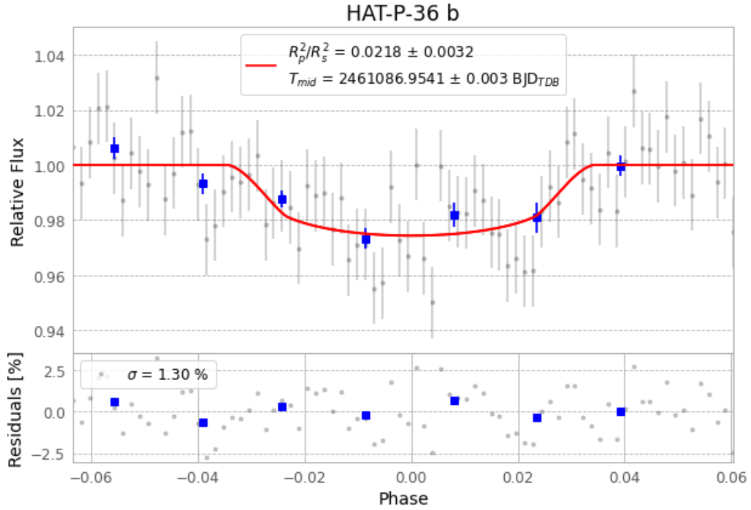
Figure 1 — FinalLightCurve_HAT-P-36 b_2026-02-15.png (SHA-256 8b6cb43c5562937a...)
