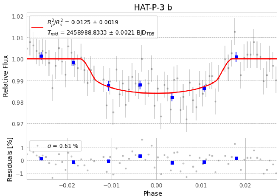
Figure 1 — FinalLightCurve_HAT-P-3 b_2020-05-18.png (SHA-256 34903e6bbcc53939...)
