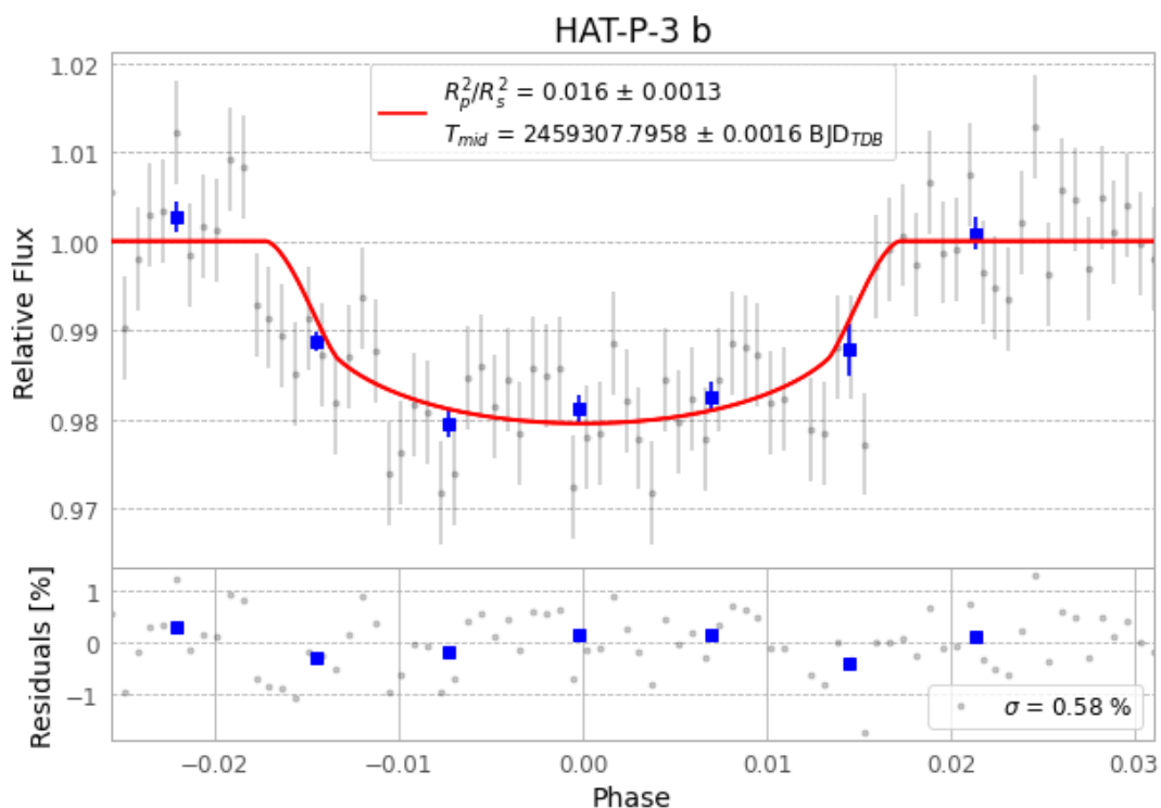
Figure 1 — FinalLightCurve_HAT-P-3 b_2021-04-02.png (SHA-256 8bd93ab229a78fb4...)
