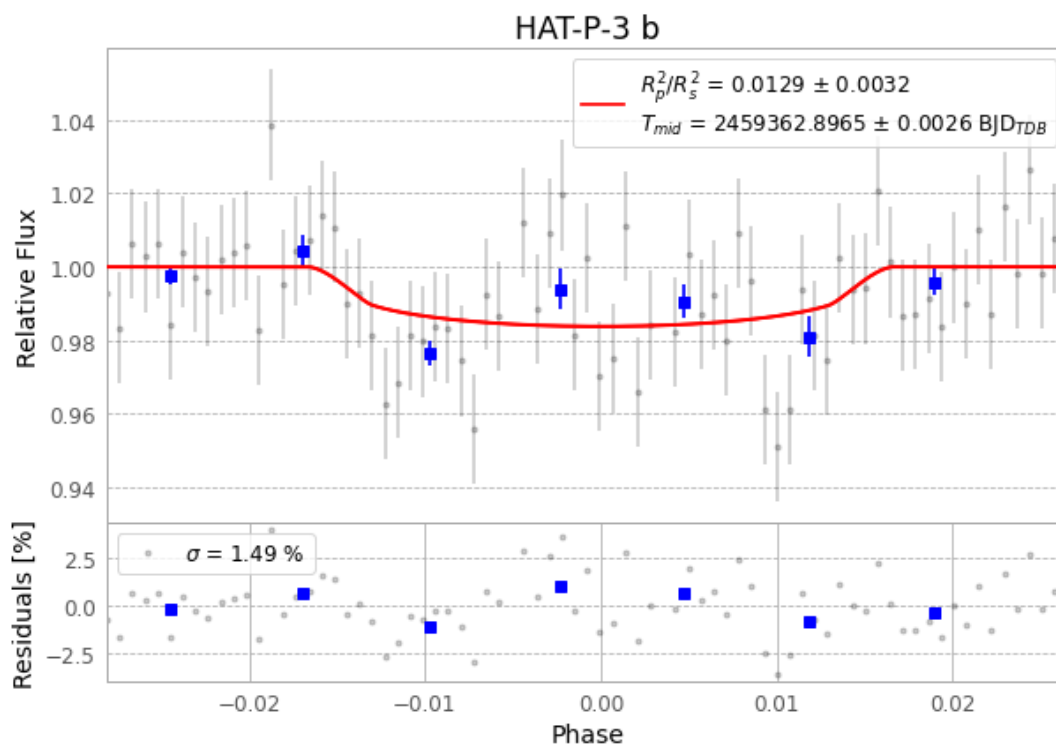
Figure 1 — FinalLightCurve_HAT-P-3 b_2021-05-28.png (SHA-256 b903dc466d3df259...)
