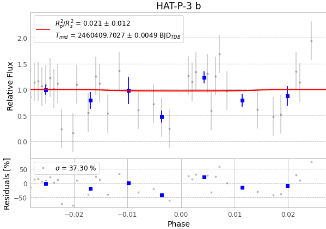
Figure 1 — FinalLightCurve_HAT-P-3 b_2024-04-08.png (SHA-256 63730959084fd1ad...)
