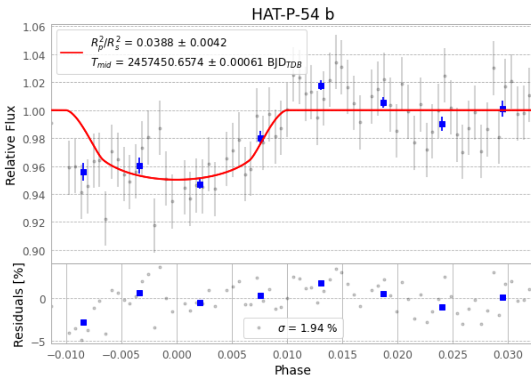
Figure 1 — FinalLightCurve_HAT-P-54 b_2016-03-02.png (SHA-256 eb7de12bfcdcbfc0...)
