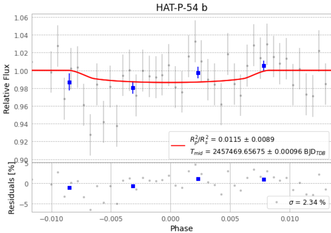
Figure 1 — FinalLightCurve_HAT-P-54 b_2016-03-21.png (SHA-256 3ee863cc51654808...)
