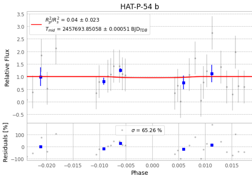
Figure 1 — FinalLightCurve_HAT-P-54 b_2016-10-31.png (SHA-256 2c724251fb78b42e...)
