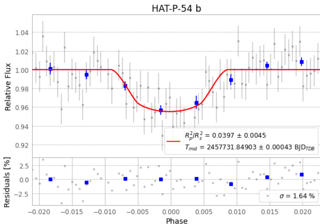
Figure 1 — FinalLightCurve_HAT-P-54 b_2016-12-08.png (SHA-256 a49f42f511db1f30...)
